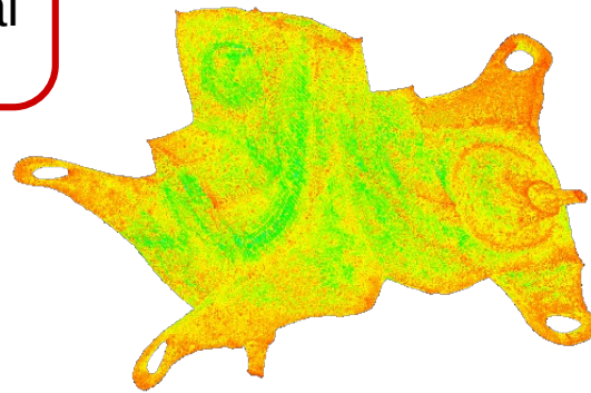
Hook1498 – 1485023 nodes
