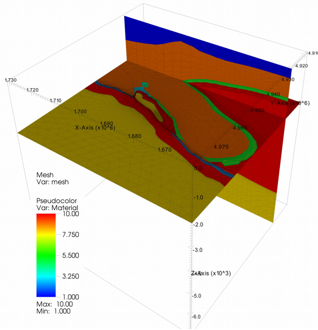
Fault simulation
