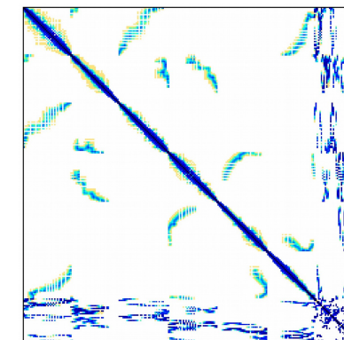
Domain Decomposition Preconditioner
