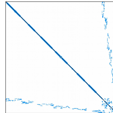
Coefficient matrix
